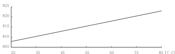
The simulation curve of wavelength varying with temperature
